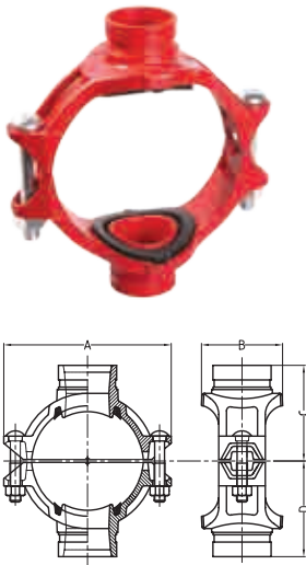
Light-duty Mechanical Cross Grooved Outlet
