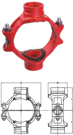
Mechanical Cross Grooved Outlet
