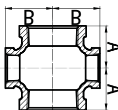
Reducing Cross
