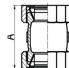
Compression Tee
