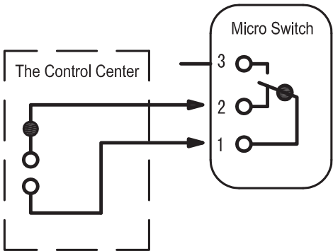
SWITCH WIRING DIAGRAM
