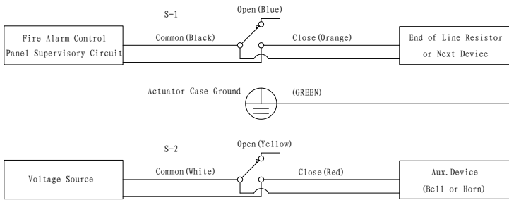
SWITCH WIRING DIAGRAM
